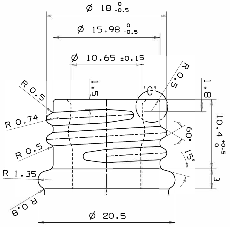
FINISH DETAILS SCALE 3:1
